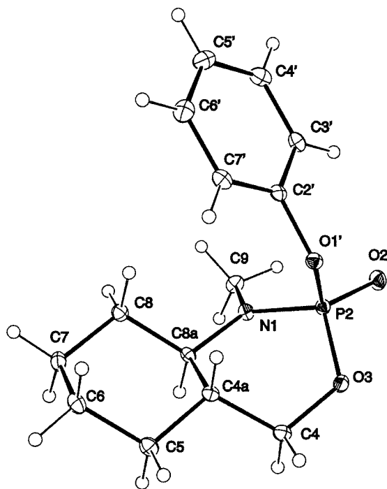
Figure 2. X-ray crystal structure of 16a .
