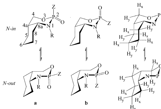
Figure 3. N-in / N-out ring inversion of epimers a and b of the cis -fused 1- R -2- Z -perhydro-3,1,2-benzoxazaphosphinine 2-oxides [R = H, Me, CH 2 Ph; Z = Ph, OPh, N(CH 2 CH 2 Cl) 2 ]. Geminal protons are labeled with subscripts x and y, H x atoms being axial in the N-in invertomer. Upon ring inversion, axial protons become equatorial and vice versa. Only chair–chair conformers are shown.
