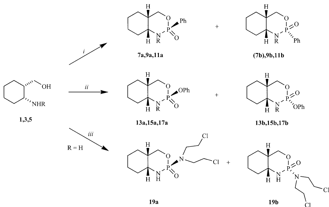
Scheme 1. Reagents: (i) Cl 2 POPh/Et 3 N in THF, column chromatography, 8–45%; (ii) Cl 2 PO(OPh)/Et 3 N in THF, column chromatography, 14–37%; (iii) Cl 2 PO[N(CH 2 CH 2 Cl) 2 ]/Et 3 N in THF, column chromatography, 30–35%. R = H: 1 , 7 , 13 ; R = Me: 3 , 9 , 15 ; R = CH 2 Ph: 5 , 11 , 17 .
