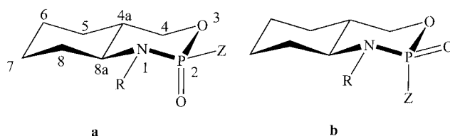
Figure 1. Diastereomers a and b of the trans -fused 1- R -2- Z -perhydro-3,1,2-benzoxazaphosphinine 2-oxides [R = H, Me, \text{CH}_2\text{Ph} ; Z = Ph, OPh, \text{N}(\text{CH}_2\text{CH}_2\text{Cl})_2 ]. Only chair–chair conformers are shown.
