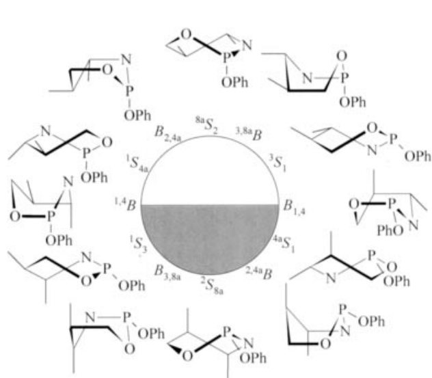
Figure 4. The idealized pseudorotational cycle for the epimers a of the trans -fused 1-R-2-OPh-perhydro-3,1,2-benzoxazaphosphinine 2-oxides. For clarity, the fused cyclohexane ring, N substituent and 2-oxo group have been omitted. The shaded area is inaccessible owing to conformational locking by the trans -fused carbocycle. The cycle is sketched for the (2 R ,4 aS ,8 aS ) enantiomers.
