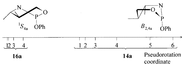
Figure 5. The nonchair conformers found for compounds 14a and 16a by a computational conformational search. The numbering of these conformers refers to that in Table 5. These closely related conformers arise mainly from the various rotameric states of the OPh substituent. The magnitude of the calculated torsion angle P2–O3–C4–H ax was used as the pseudorotational coordinate.
