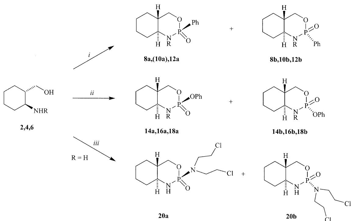
Scheme 2. Reagents: (i) \text{Cl}_2\text{POPh}/\text{Et}_3\text{N} in THF, column chromatography, 10–37%; (ii) \text{Cl}_2\text{PO(OPh)}/\text{Et}_3\text{N} in THF, column chromatography, 16–42%; (iii) \text{Cl}_2\text{PO}[\text{N}(\text{CH}_2\text{CH}_2\text{Cl})_2]/\text{Et}_3\text{N} in THF, column chromatography, 63%. R = H: 2 , 8 , 14 ; R = Me: 4 , 10 , 16 ; R = \text{CH}_2\text{Ph} : 6 , 12 , 18 .
